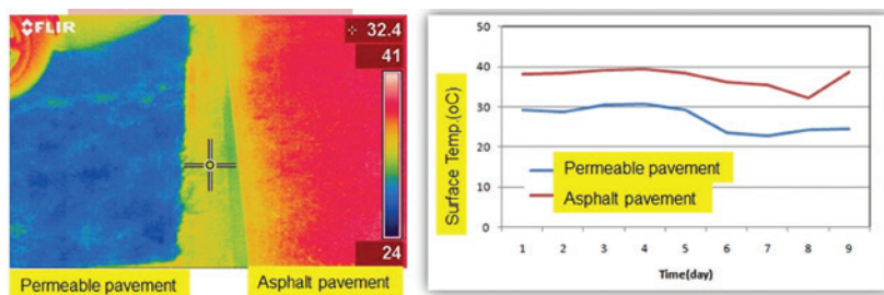
Figure 10.9 Surface temperature reduction by permeable pavement.
